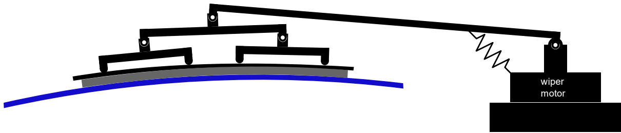
Picture 8 - Later design of windshield wiper on curved glass
