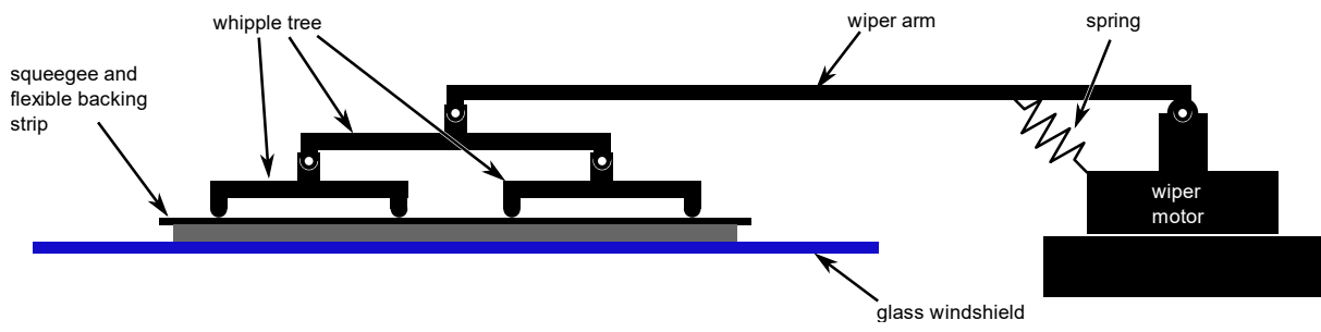
Picture 7 - Later design of windshield wiper on flat glass
